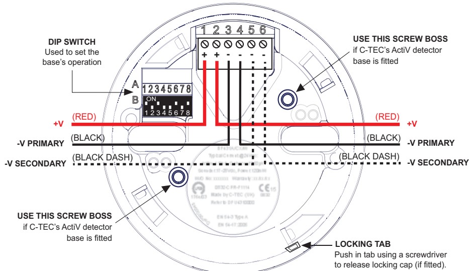
Figure 1 - Sounder Connections (Typical)
