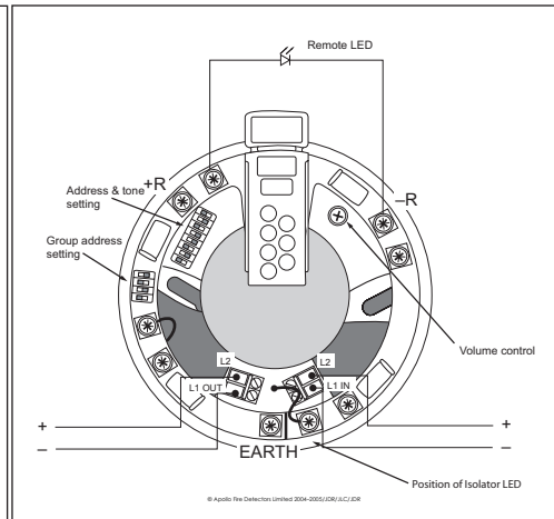
Fig. 3 Integrated Base Sounder with isolator wiring
